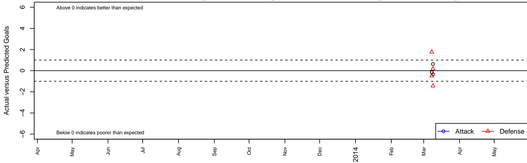
Heat FC 96 LS B95 Dots are actual minus expected GF (blue circles) and GA (red triangles). Blue line is smoothed change in attack strength. Red is smoothed change in defense strength.
